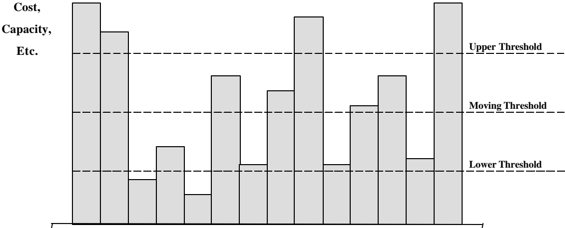
Fig. 2 All Costs (or Capacities, Resource Levels, etc.) Above – or Alternately Below – the Moving Threshold are Treated as if Equal the Threshold Value
