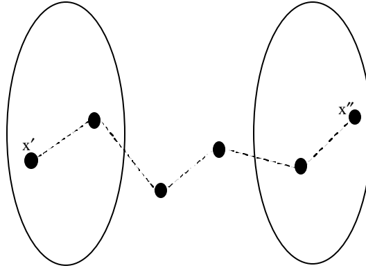
Fig. 5 Feasible region consists of disconnected components. The path “tunnels through” the infeasible region to regain feasibility.
