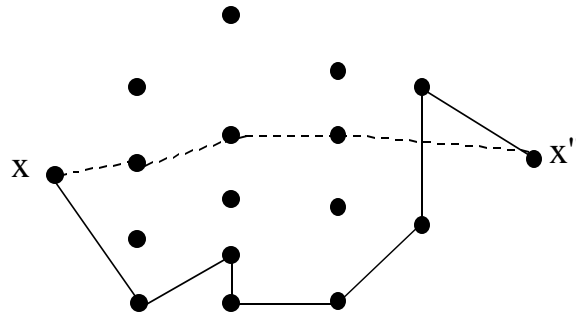
Fig. 3 Path relinking. Original path shown by heavy line; relinked path (one possibility) shown by dotted line
