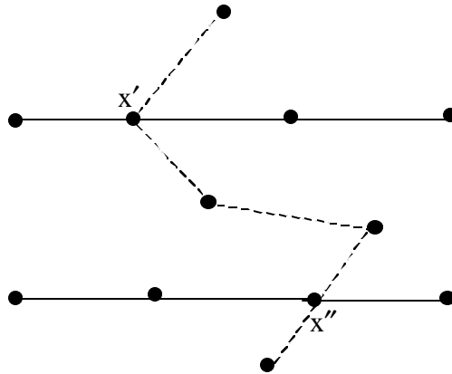
Fig. 4 Path Relinking: Previously generated paths shown by heavy lines; relinked path shown by dotted line. (Multiple additional points in the space are not shown.)
