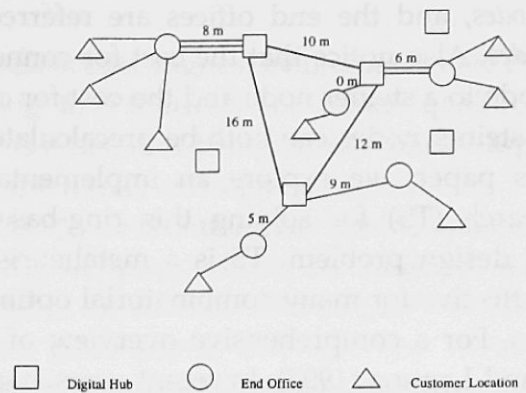
Figure 1 A Ring-Based DDS Network
